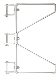
Steel galvanized Standoff 18" from pole SP-6275-GLV
