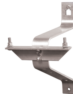
Aluminum standoff cutout and arrestor mount, standoff 17" from pole SP-6092
