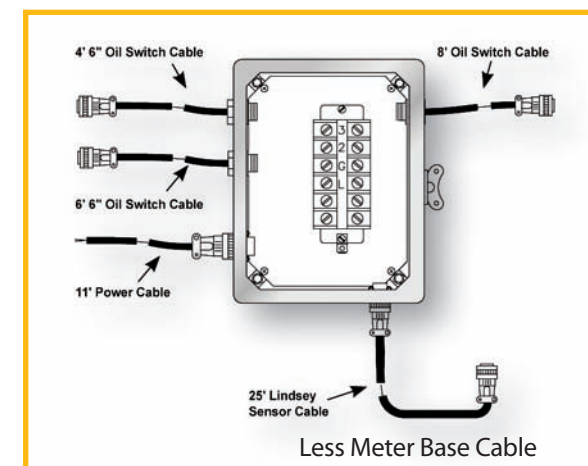
Less Meter Base and Sensor Cables
