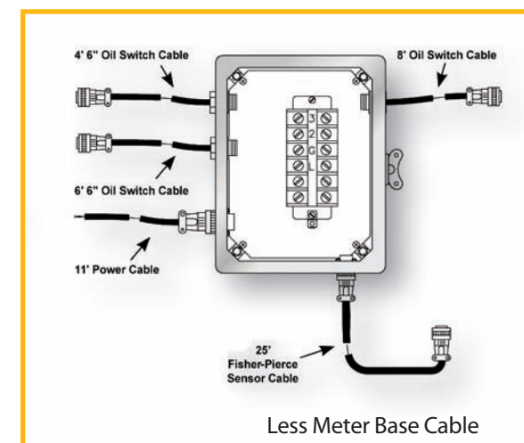
Less Meter Base Cable
